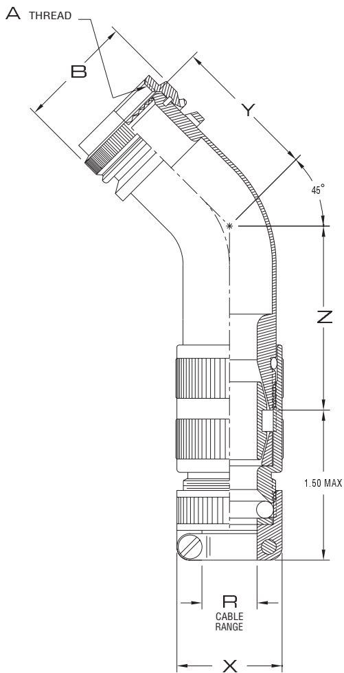
45° BODY STYLE
