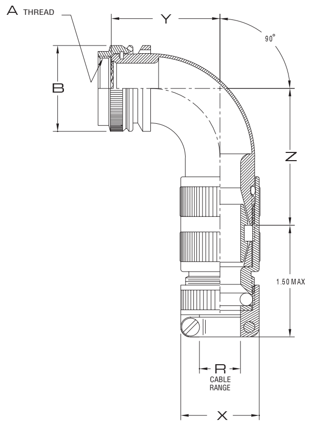
90° BODY STYLE
