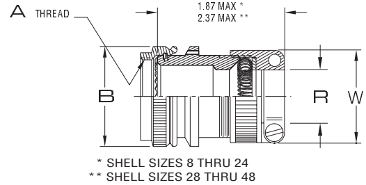
FIGURE 4: Completed Assembly of individual shields terminated with Iris Adapter.
