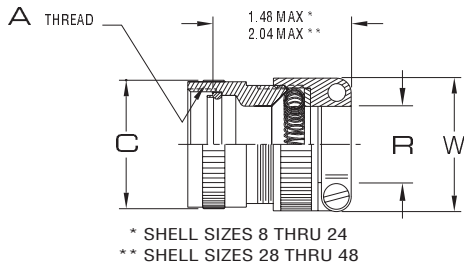
FIGURE 2: Individual Shield Adapter Body assembled to connector, shields dressed through the Iris.
